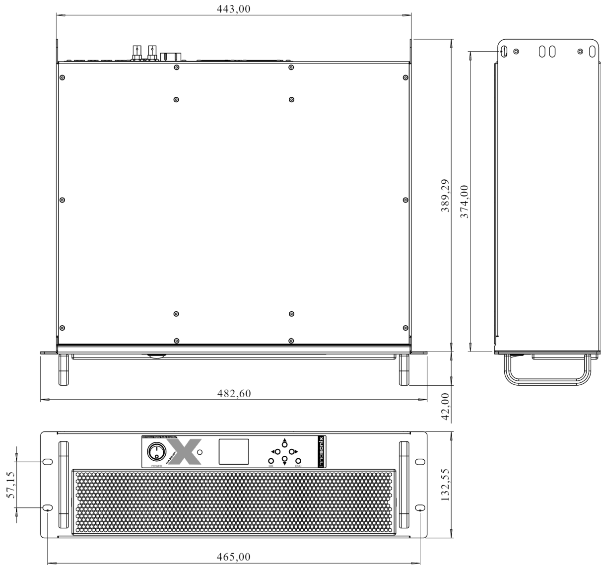
Figure 1. MAXX/HP 2 dimensions
